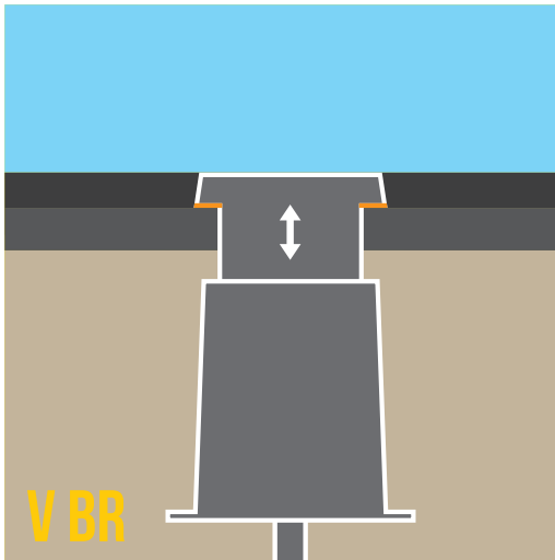
V BR Ideal tarmac installation for very robust application areas
